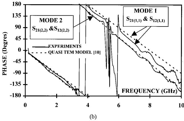
Fig. 7. Generalized scattering parameters of a delay line. (a) Magnitude of the 16 S -parameters. (b) Phase of the four nonnull parameters appearing in (32).
